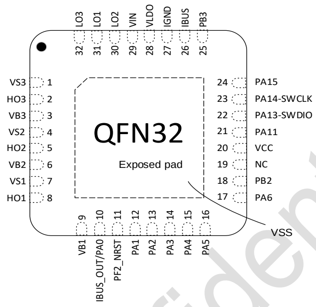
图 3-1 QFN32(4*4) Pinout1 PY32MD320K1xU7 (Top View)
